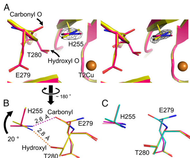
Fig. 2. Conformational change of His255 (molecule A). (A) The sigma-A-weighted 2F o -F c maps (3.0 σ, gray) around His255 in the SFX RS structure (Left) and the SRX RS structure (Right). (B) Switching of H-bond partners. The SFX RS and SRX RS structures are shown in pink and yellow, respectively. Dashed lines represent H-bonds. (C) Comparison of the His255 conformation. The SRX RS, SFX NC, and SRX NC structures are shown in yellow, magenta, and cyan, respectively. The SFX RS structure is shown in light pink.
