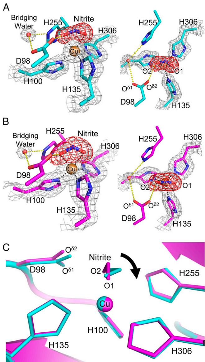
Fig. 1. NO 2 - binding in NC structures. (A) T2Cu site in the SRX NC structure (molecule A). The sigma-A-weighted 2F o -F c (1.5 σ) and omit F o -F c (6.5 σ) maps are shown as gray and red meshes, respectively. H-bonds (yellow) and coordination bonds (black) are represented by dashed lines. C, N, O, and Cu atoms are colored cyan, blue, red, and brown, respectively. (B) T2Cu site in the SFX NC structure (molecule A). The sigma-A-weighted 2F o -F c (1.0 σ) and omit F o -F c (4.5 σ) maps are shown as gray and red meshes, respectively. H-bonds and coordination bonds are represented as in A. C, N, O, and Cu atoms are colored magenta, blue, red and brown, respectively. (C) Comparison between the SFX NC (magenta) and SRX NC (cyan) structures.
